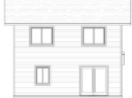
REAR ELEVATION SCALE: 1/4" = 1'-0"
